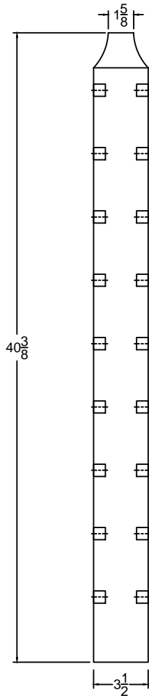
SECTION VIEW
