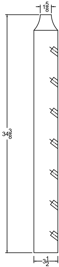
SECTION VIEW
