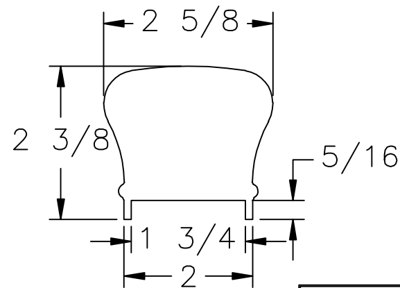
LJ-6210 PROFILE
