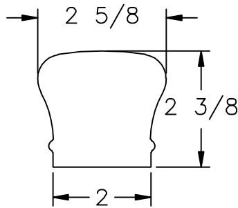
LJ-6210 PROFILE
