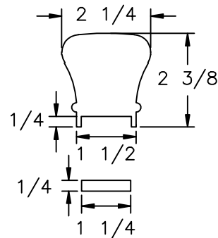
LJ-6010 PROFILE
