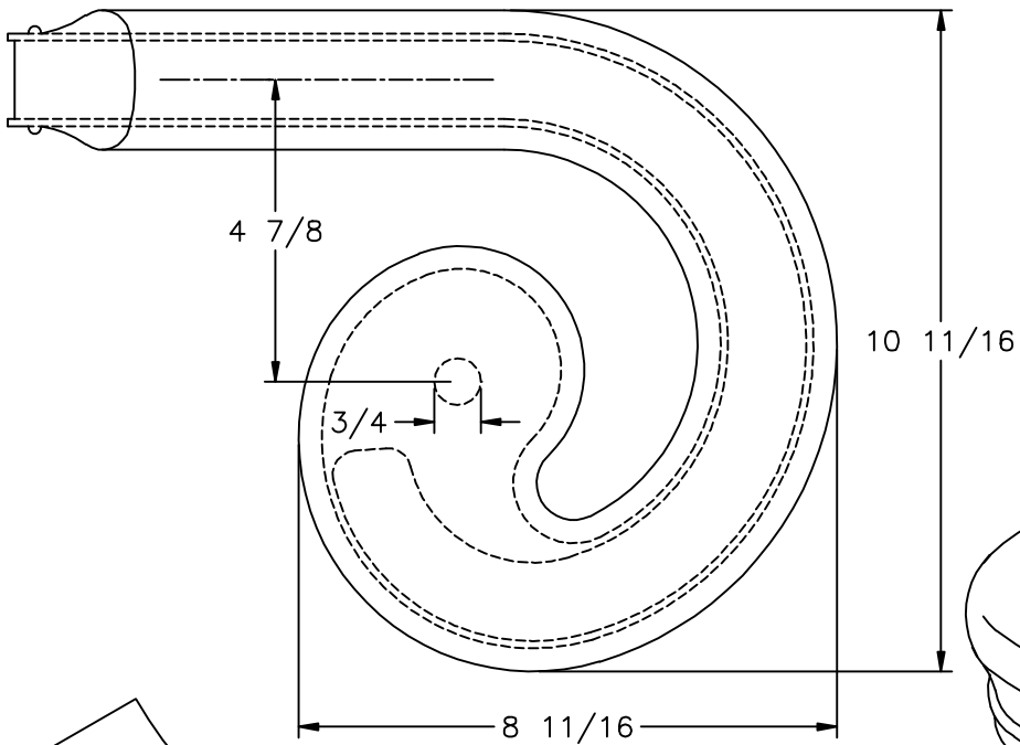
LJ-6010 PROFILE
