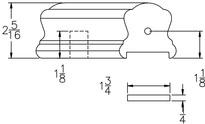
LJ-6B10 PROFILE
