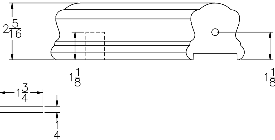
LJ-6B10 PROFILE
