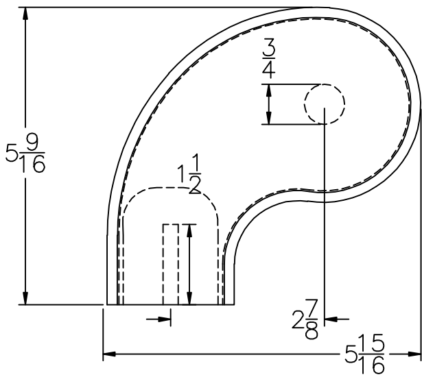
LJ-6B10 PROFILE
