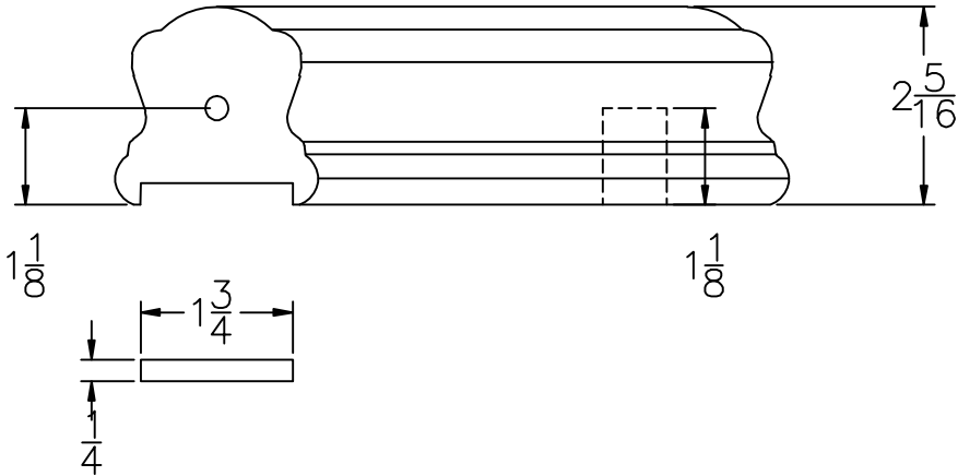
LJ-6B10 PROFILE
