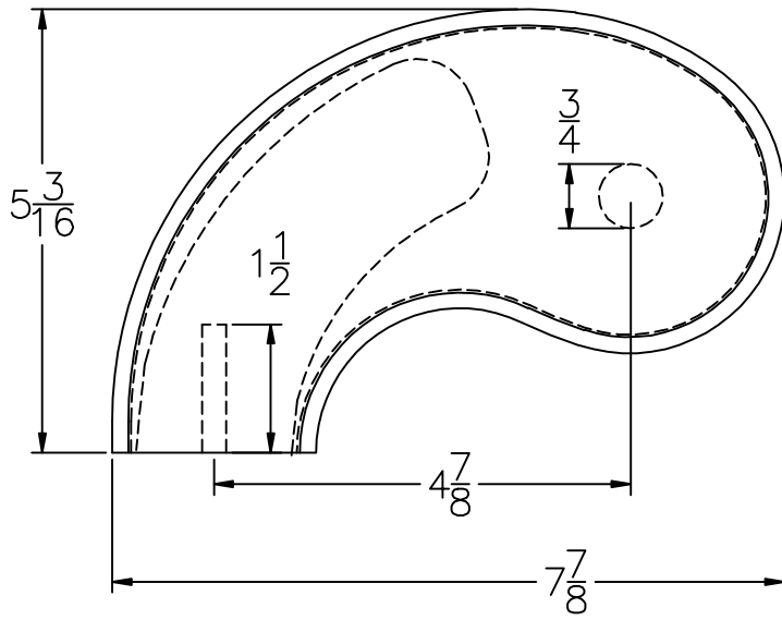
LJ-6B10 PROFILE
