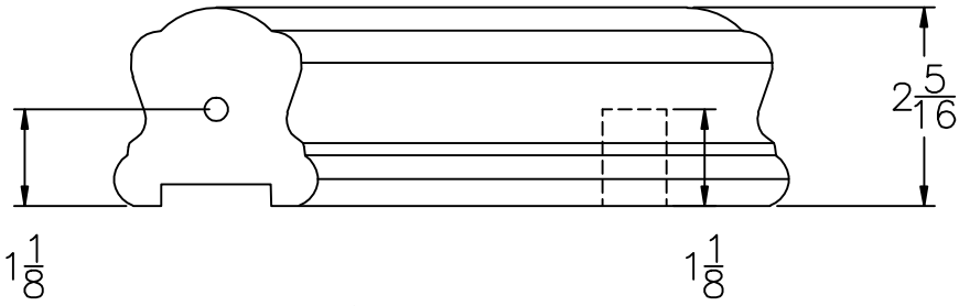
LJ-6B10 PROFILE
