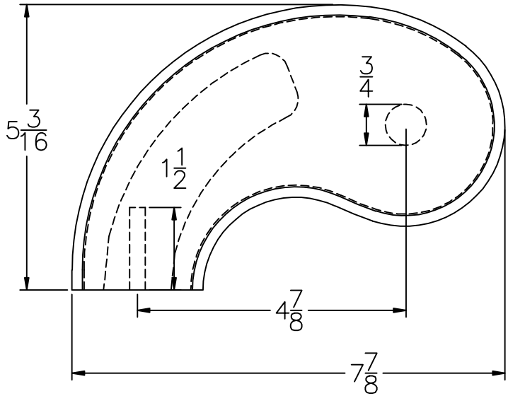
LJ-6B10 PROFILE
