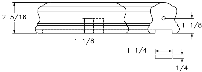
LJ-6B10 PROFILE
