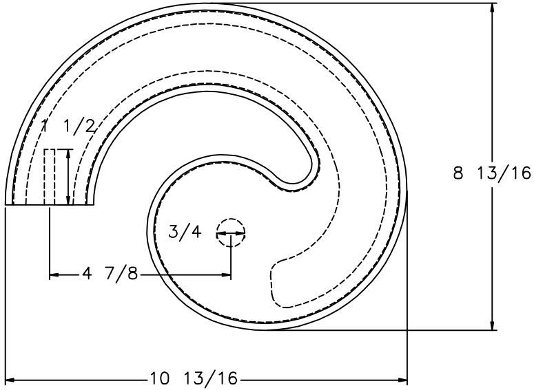
LJ-6B10 PROFILE
