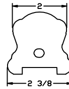
LJ-6B10 PROFILE
