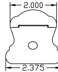
LJ-6B10 PROFILE
