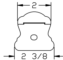
LJ-6B10 PROFILE
