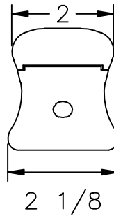
LJ-6A10 PROFILE
