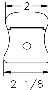
LJ-6010 PROFILE
