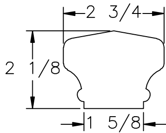
LJ-6701 PROFILE
