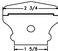
LJ-6701 PROFILE
