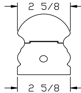
LJ-6519 PROFILE
