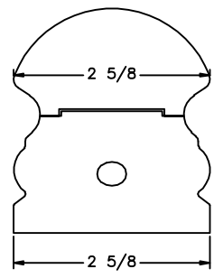
LJ-6519 PROFILE
