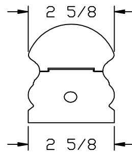
LJ-6519 PROFILE
