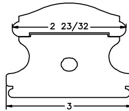
LJ-6400 PROFILE
