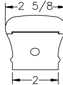
LJ-6210 PROFILE
