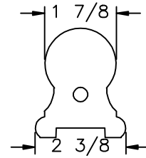
LJ-6109P0 PROFILE
