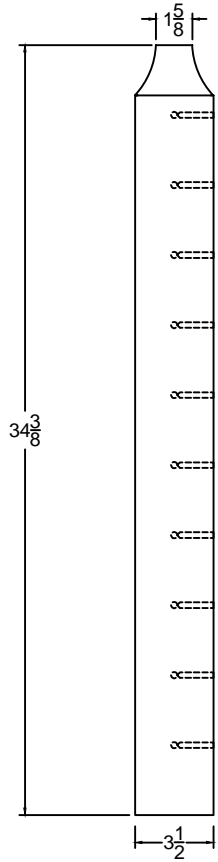
SECTION VIEW
